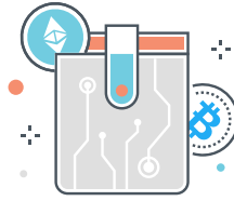
ETHEREUM WALLETS
