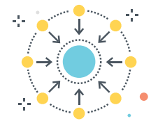
DECENTRALIZED MINING
