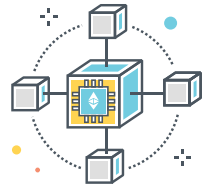
ETHEREUM BLOCKCHAIN
