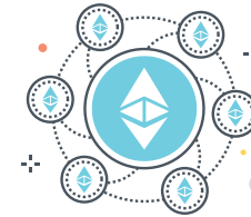
AUTOMATIC DISTRIBUTION
